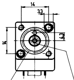
0-Ring 12 x 1.5 Connection P 0-Ring 3 x 1.5
